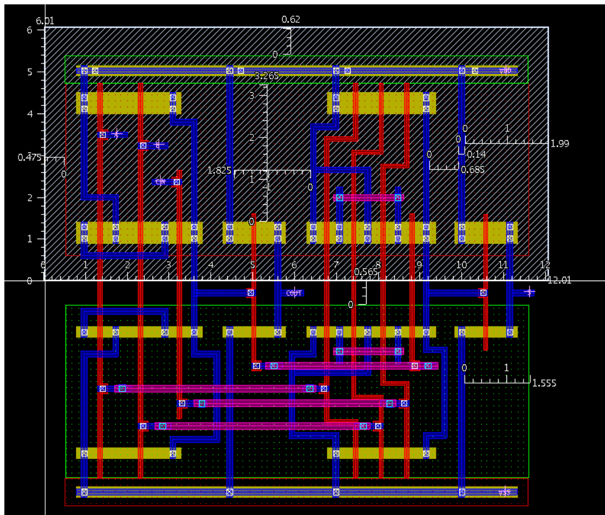
Figure 2: 1-bit Full Adder Layout
