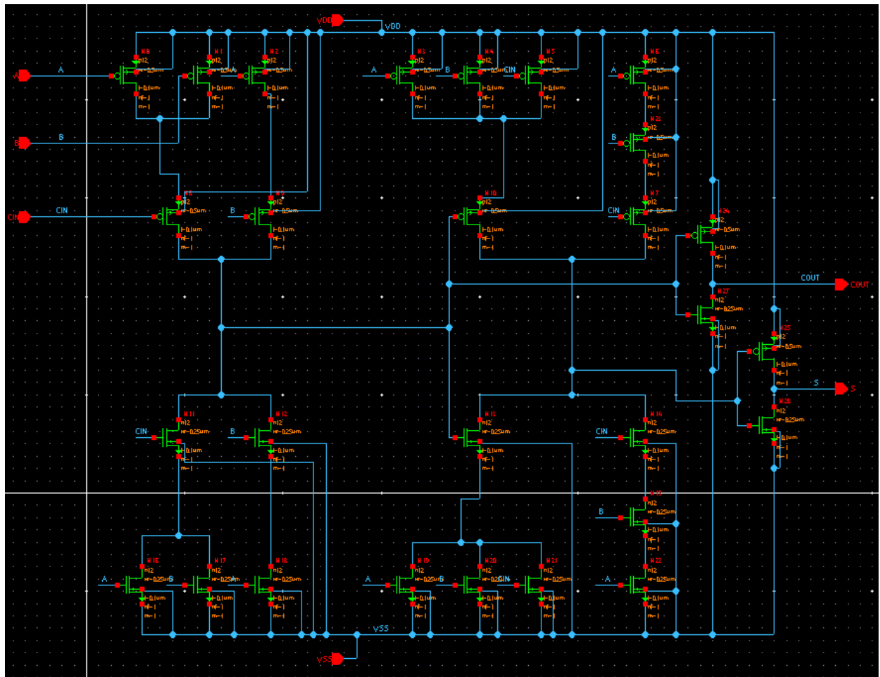
Figure 1: 1-bit Full Adder Schematic
