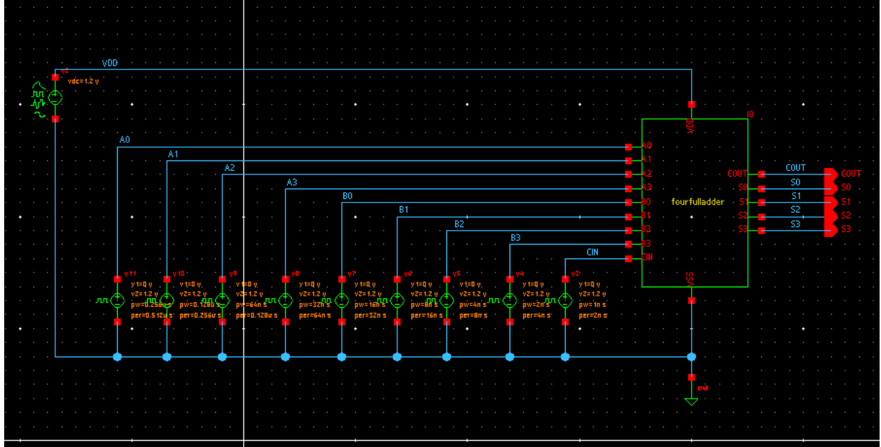
Figure 10: 4-bit Full Adder Testbench Schematic
