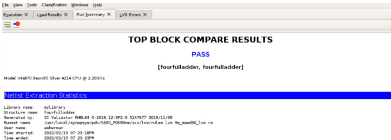
Figure 9: 4-bit Full Adder LVS Results
