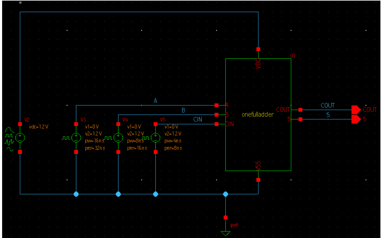
Figure 5: 1-bit Full Adder Testbench Schematic
