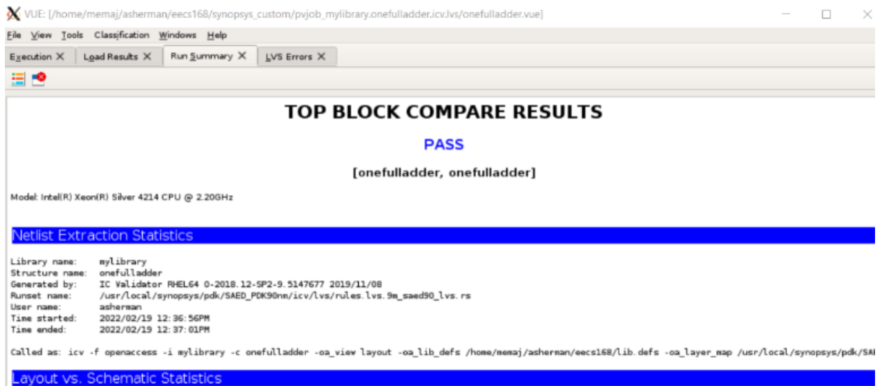
Figure 4: 1-bit Full Adder LVS Results
