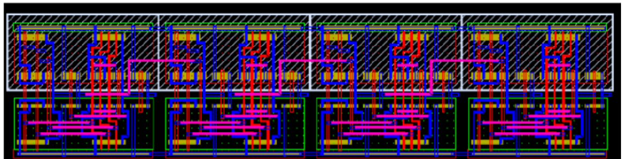
Figure 7: 4-bit Full Adder Layout
